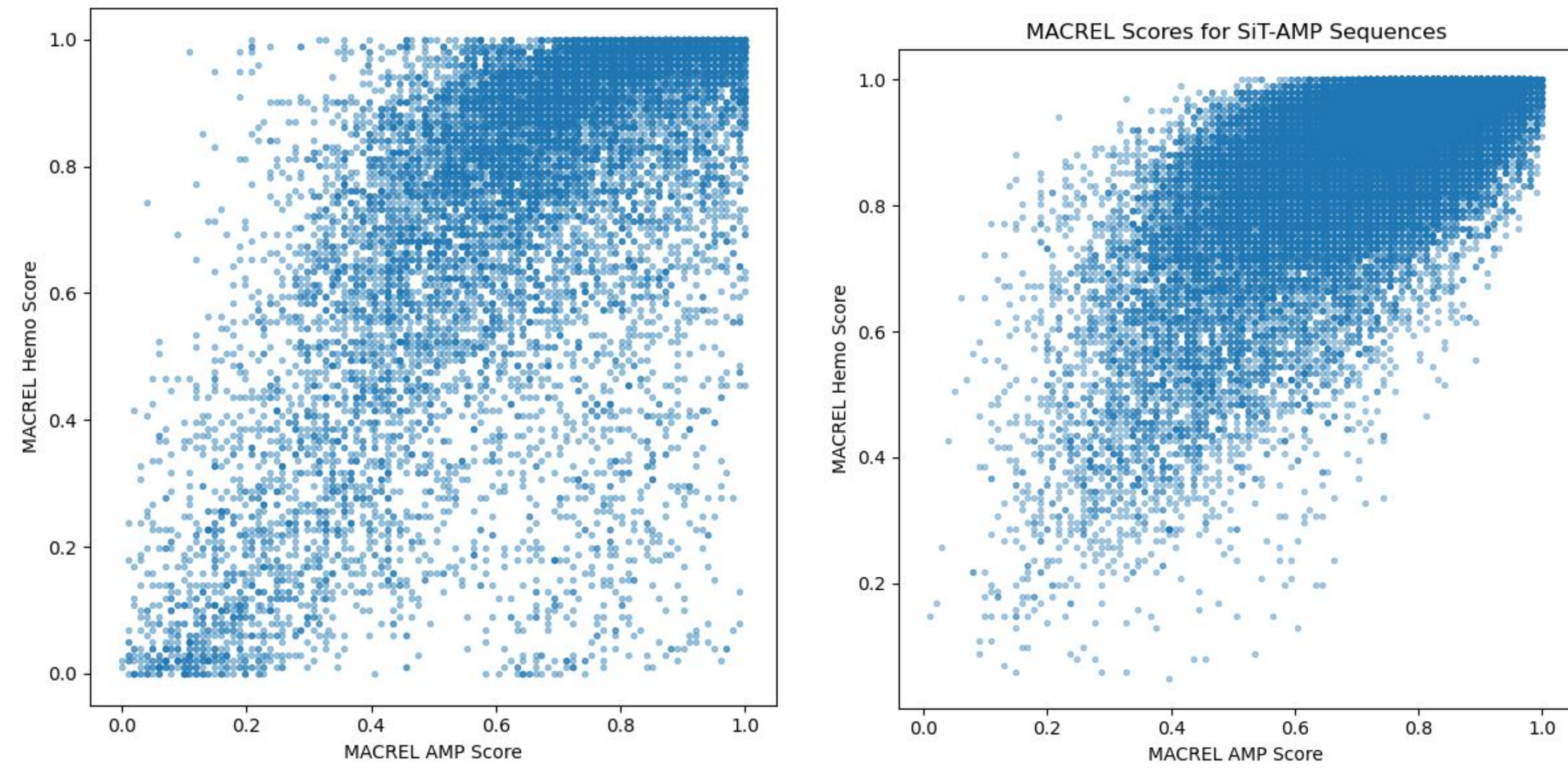
Training and sampling Macrel values distribution (left: Training, Right: Sampling)
